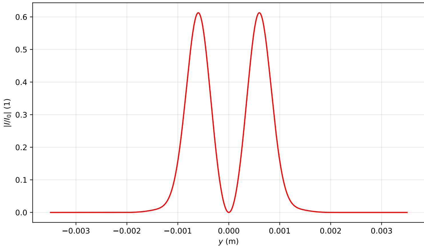
Intensity profile I(x=0, y, z=1.115)/I_0 , P_{in}=2.0P_{cr} , artificial time
